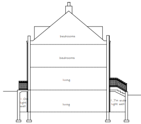
SECTION
